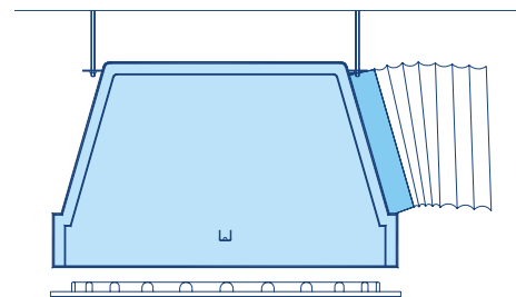
Aircobox 600 - diameter 200
