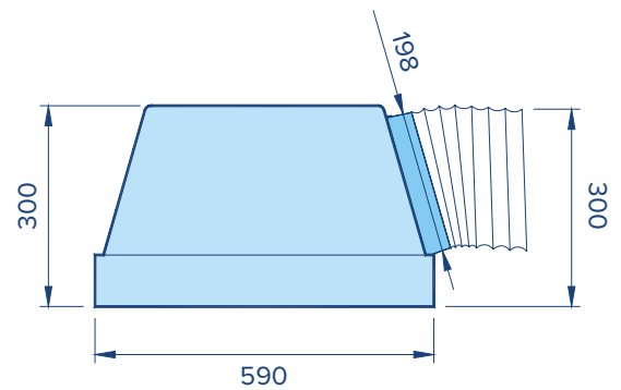
Aircobox 600 - diameter 200
